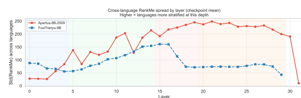
Figure 13: Cross-language standard deviation of RankMe at each layer (H2), both models. FuxiTranyu peaks at layer 15 (the semantic-building/compression boundary); Apertus at layer 21.
